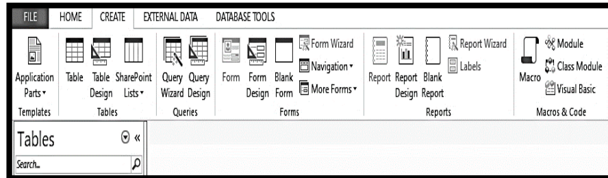
Figure 232: Create tab
