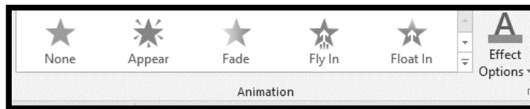
Figure 207: Animations group
