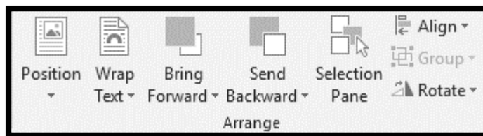
Figure 188: Arrange Group
