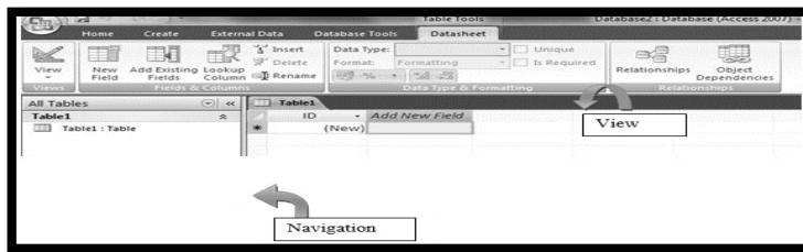
Figure 230: Blank Database
