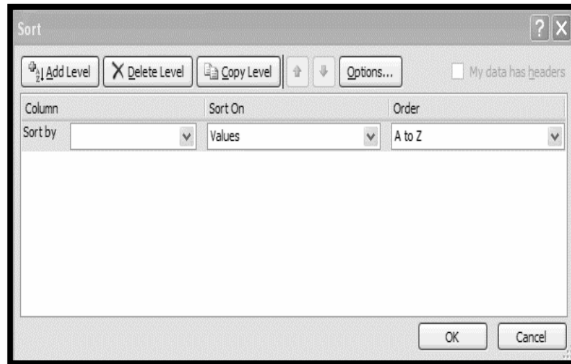
Figure 226: Custom Sort
