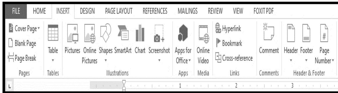
Figure 158: Inert tab
