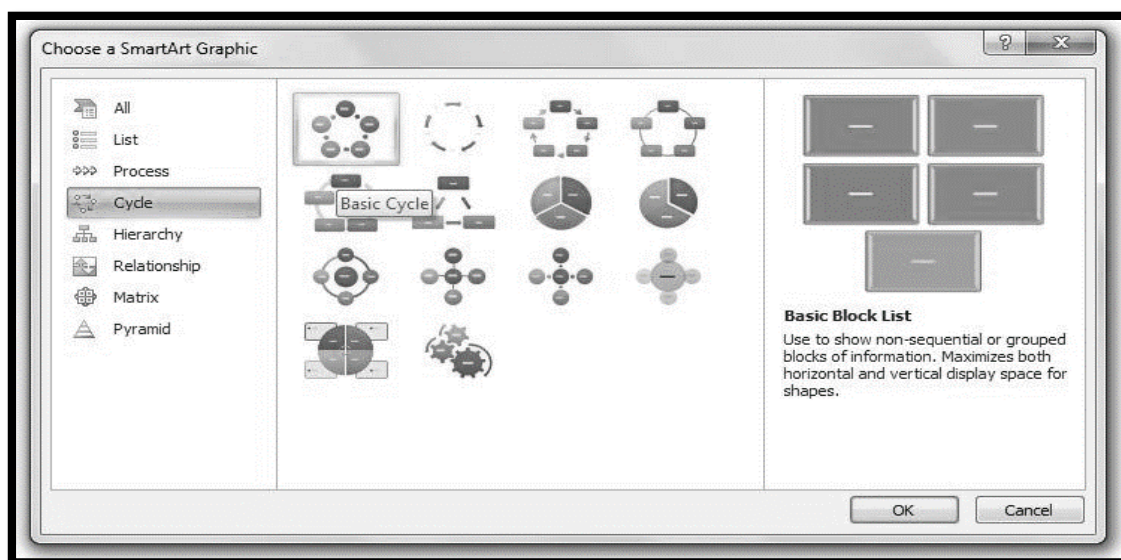
Figure 169: Basic cycle
