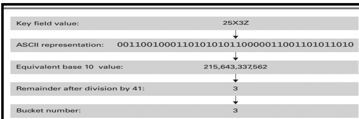
Figure 121: Hashing the key field value 25X3Z to one of 41 buckets
