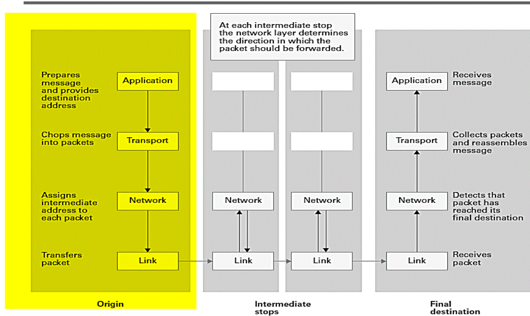
Figure 75: Following a message through the Internet
