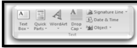
Figure 178: Text group
