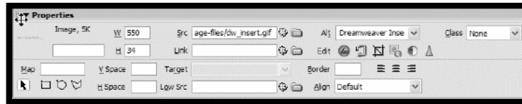
Figure 247: Properties panel
