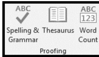
Figure 191: Proofing group
