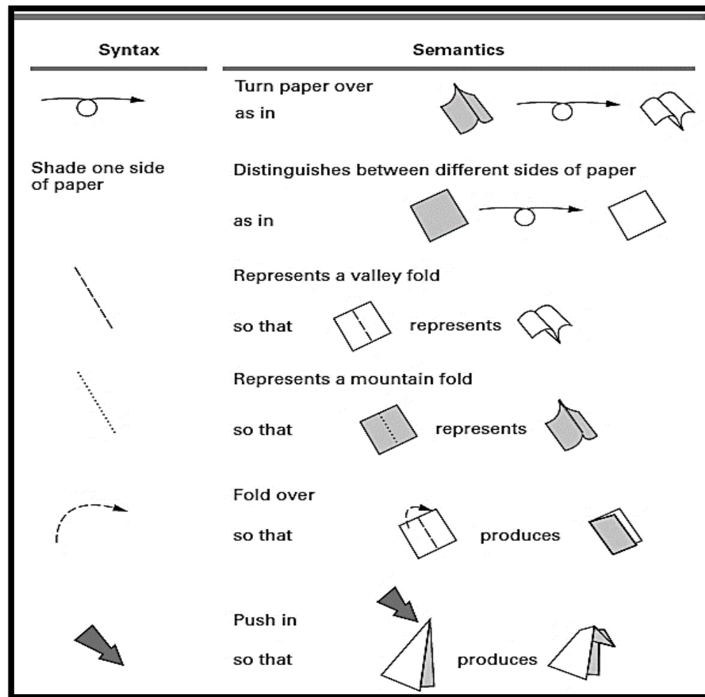
Figure 79: Origami primitives
