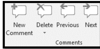
Figure 193: Comments group
