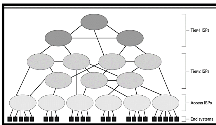
Figure 65: Internet composition
