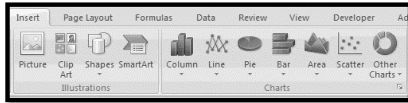
Figure 211: Charts group
