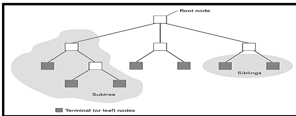
Figure 106: Tree terminology
