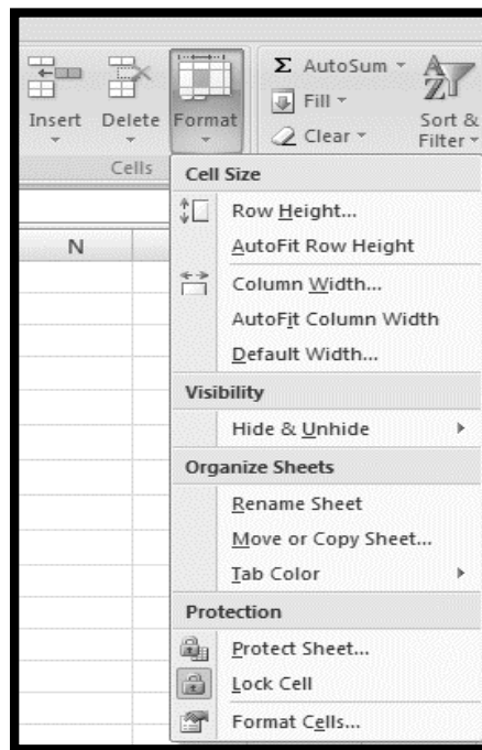
Figure 210: Cell formatting
