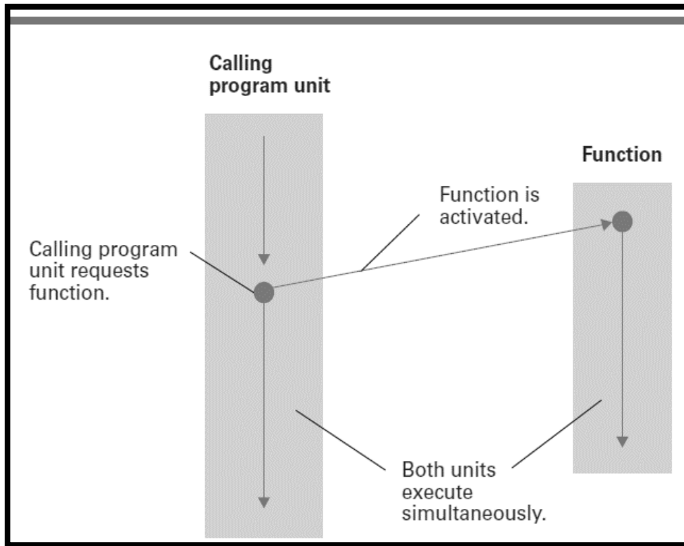
Figure 96: Spawning threads
