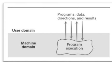
Figure 51: Interactive Processing
