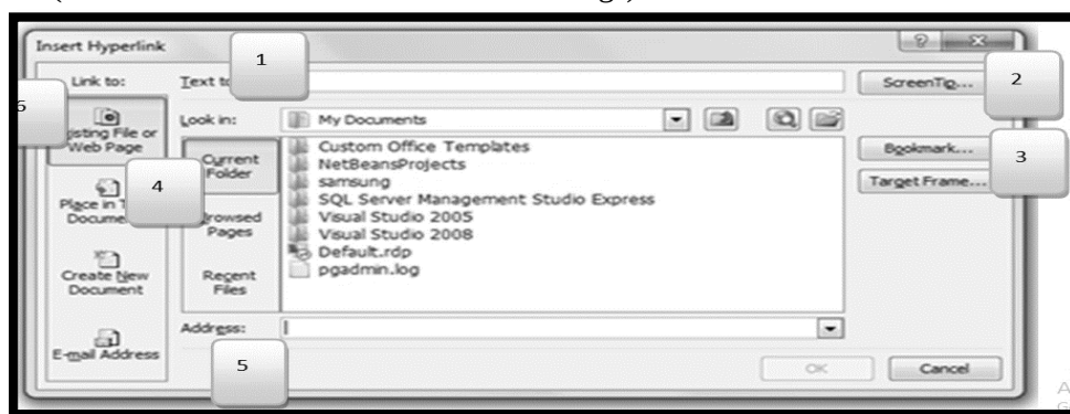
Figure 173: Adding Hyperlink
