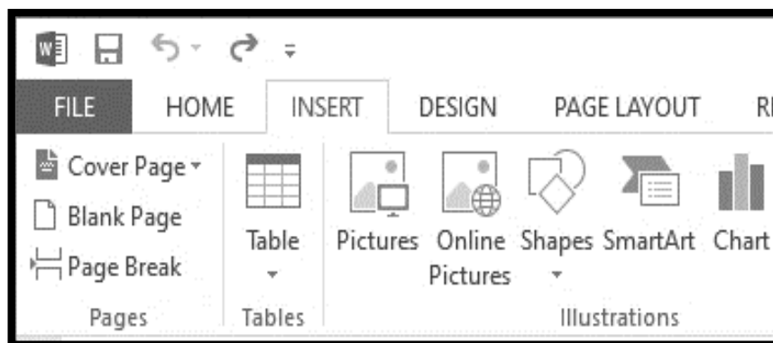
Figure 164: Illustrations
