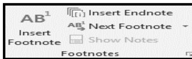
Figure 190: Footnotes Group
