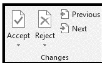
Figure 195: Changes group
