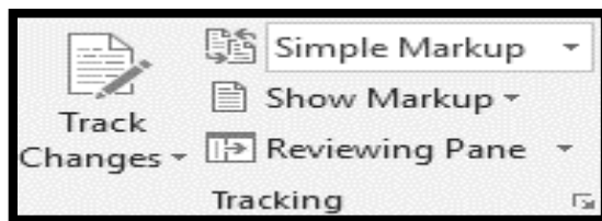
Figure 194: Tracking group
