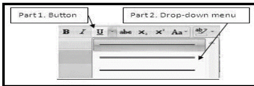
Figure 136: Underline Panel
