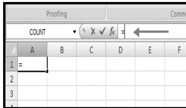
Figure 213: Formula Example
