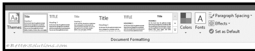
Figure 182: Design Ribbon
