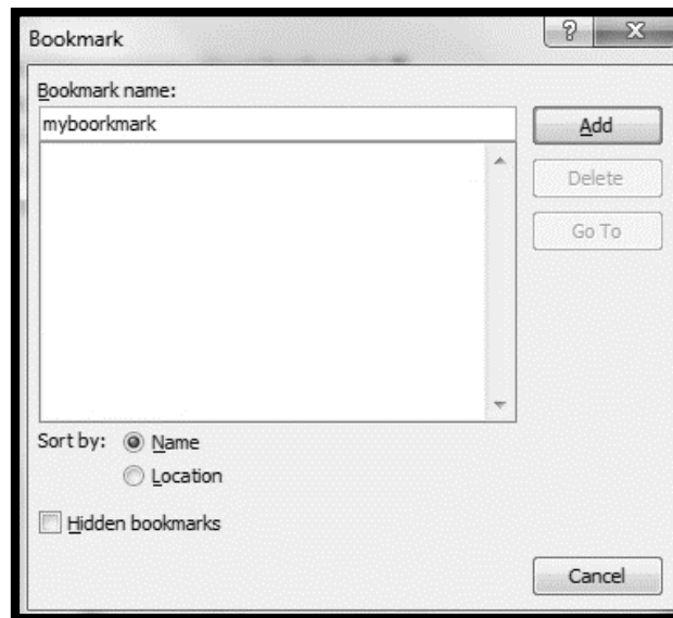
Figure 174: Adding Bookmark
