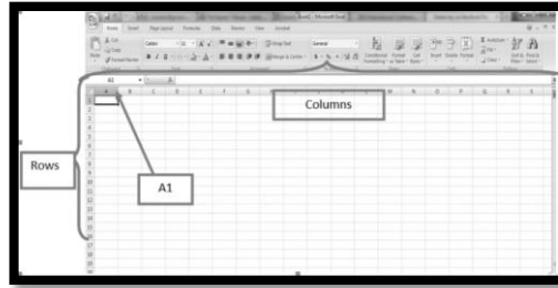
Figure 209: Excel Layout
