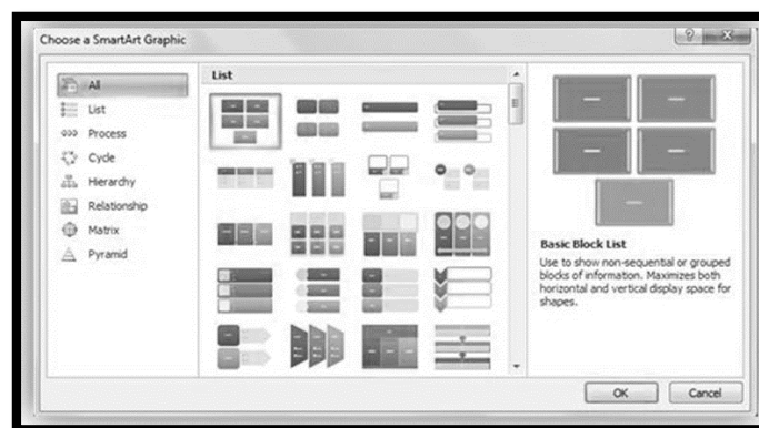
Figure 168: Smart Art
