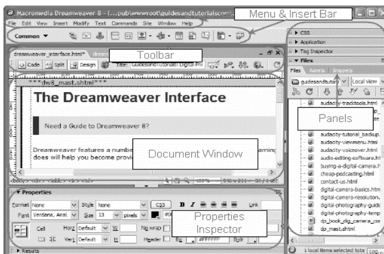
Figure 246: Dreamweaver interface
