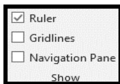
Figure 199: Show group
