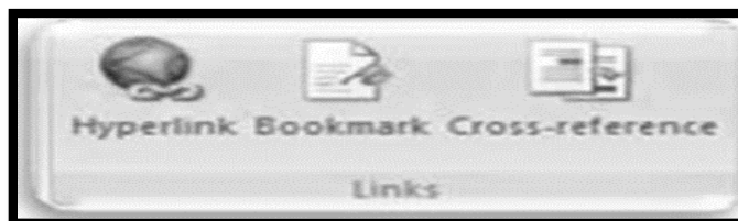
Figure 172: Links group
