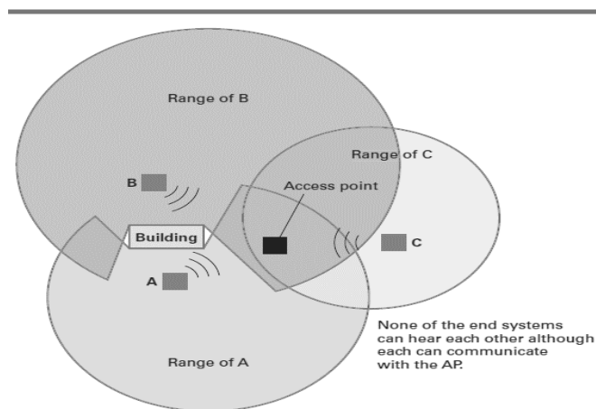
Figure 61: The hidden terminal problem
