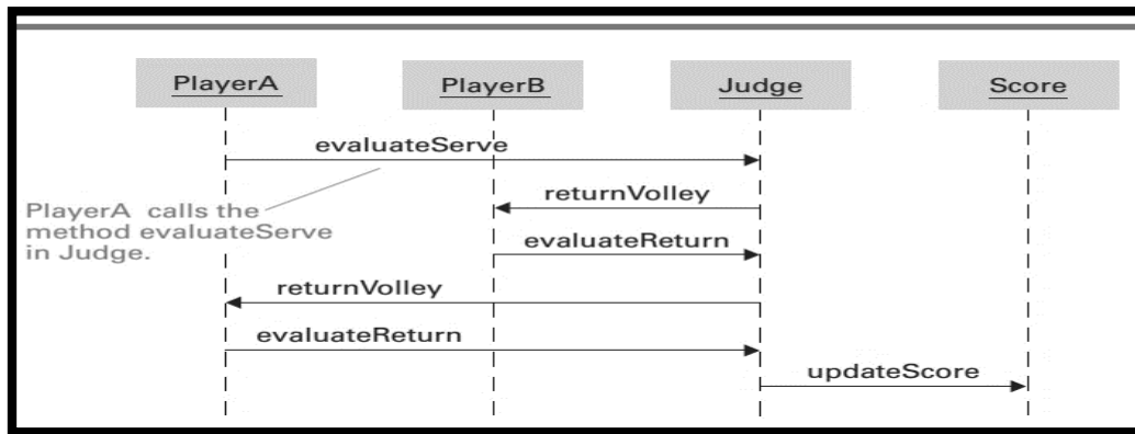
Figure 100: The interaction between objects resulting from PlayerA's serve.
