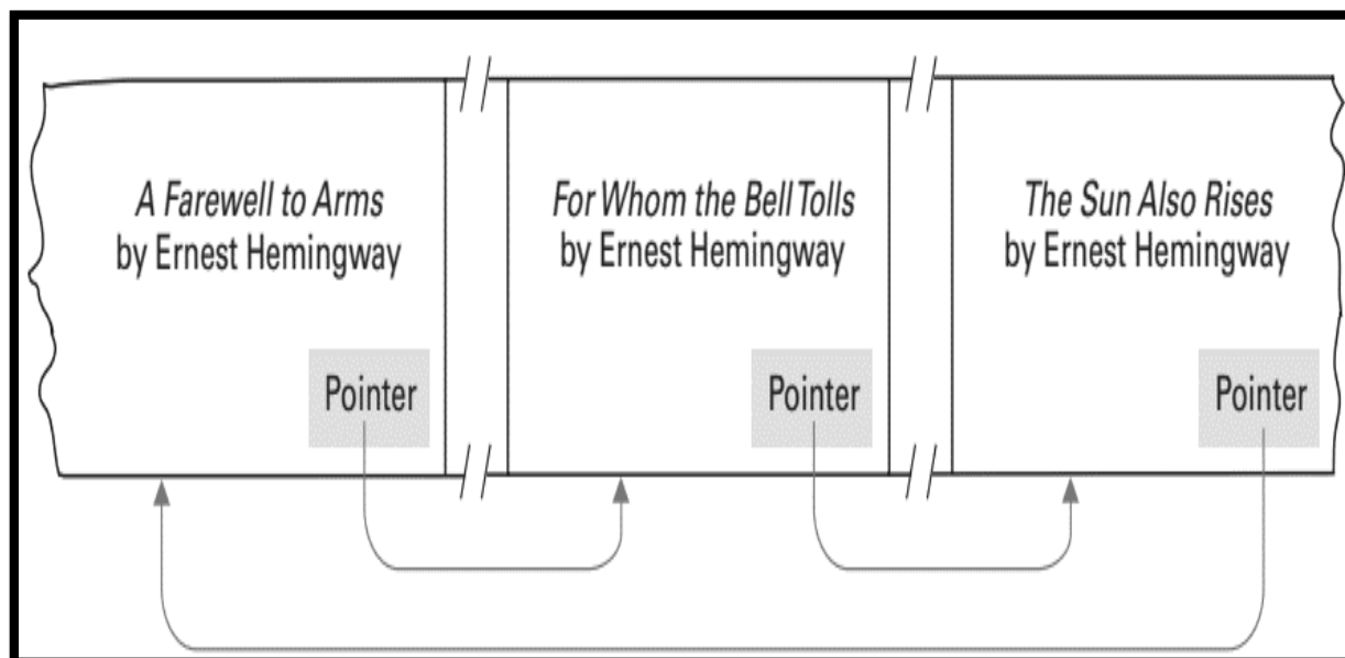
Figure 107: Novels arranged by title but linked according to authorship
