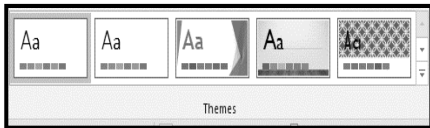
Figure 204: Themes group
