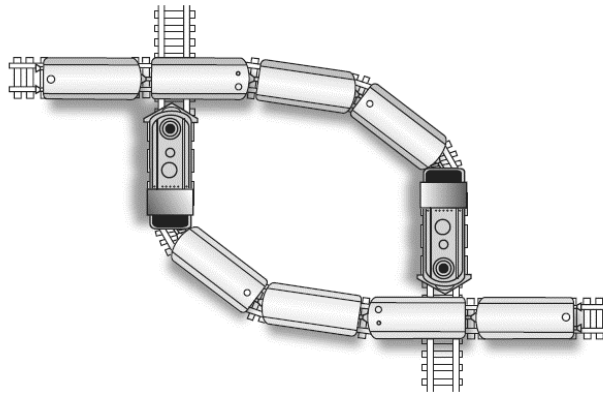
Figure 58: Deadlock Situation
