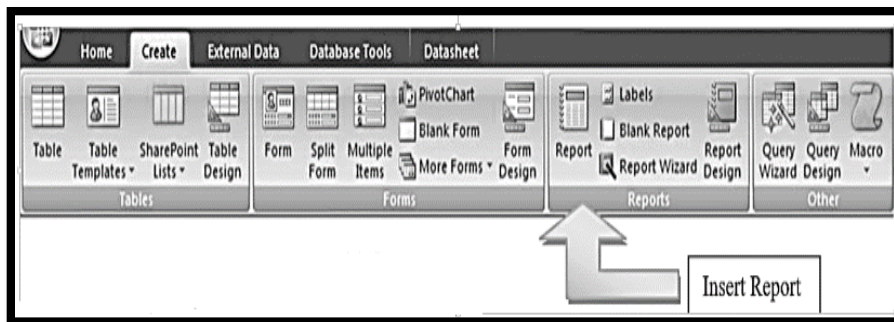
Figure 234: Insert Report
