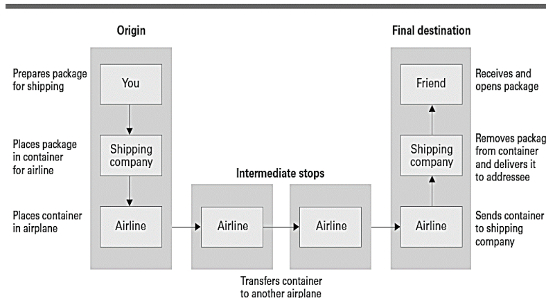
Figure 73: Package-shipping example
