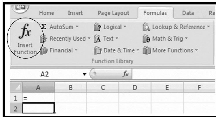
Figure 218: Function Computation
