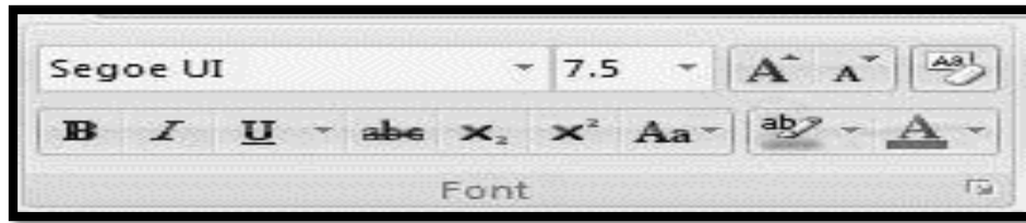
Figure 146: Font group
