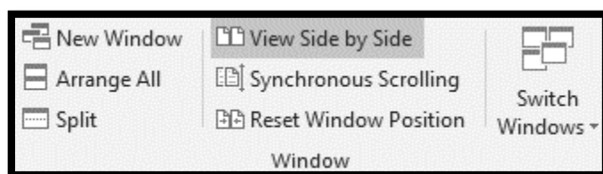
Figure 201: Windows group
