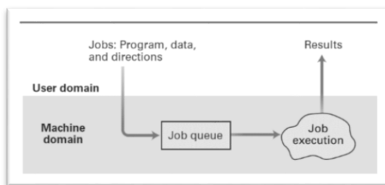
Figure 50: Batch Processing
