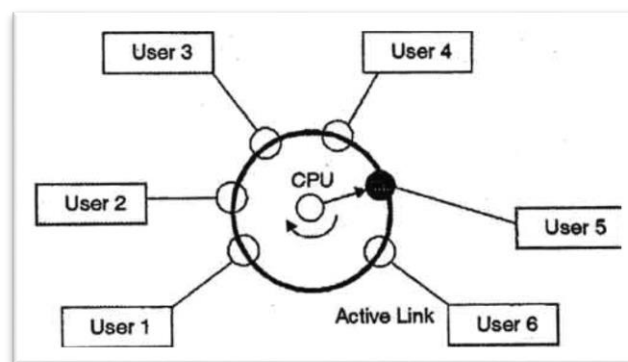
Figure 52: Time Sharing
