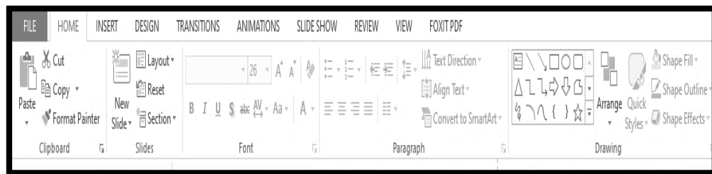
Figure 202: MS: Powerpoint
