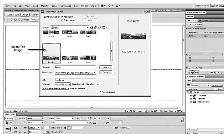
Figure 257: Browse Image
