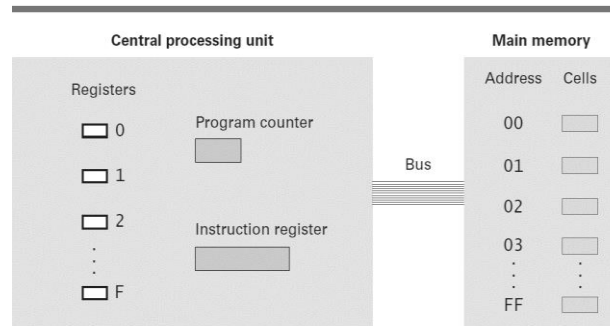
Figure 43: CPU and Main memory linkage using Bus
