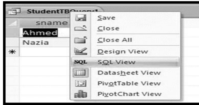
Figure 239: SQL View
