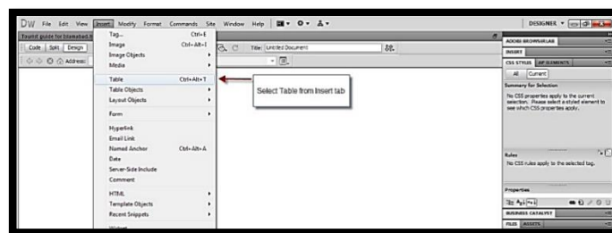
Figure 251: Insert Table
