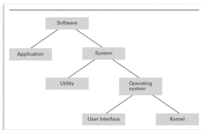
Figure 53: Software Classification
