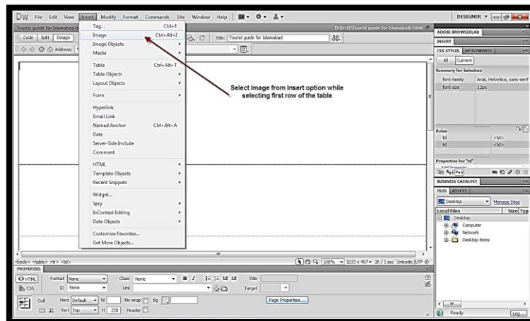
Figure 256: Inserting Image
