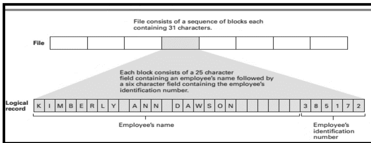
Figure 119: The structure of a simple employee file implemented as a text file
