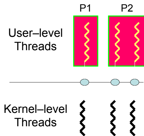
Figure 13.2 One-to-One Model
