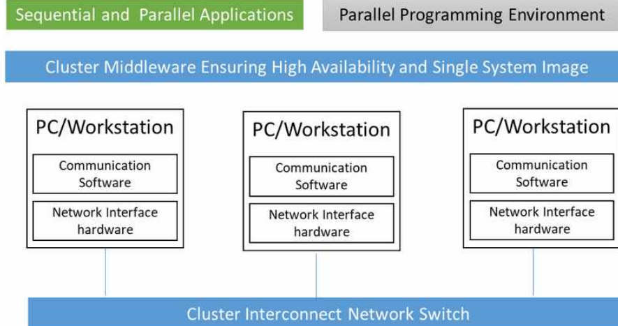
Cluster Architecture
