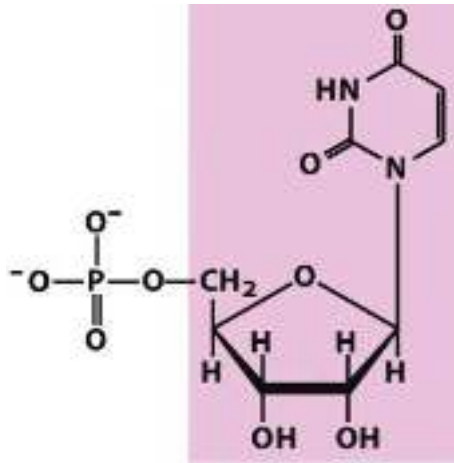
Uridylate (uridine 5'-monophosphate)
