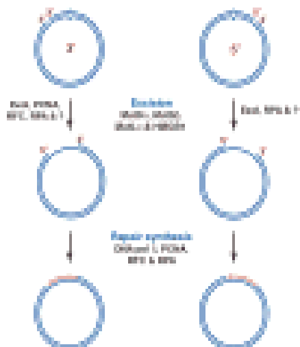
Substrates and requirements for in vitro mismatch repair
